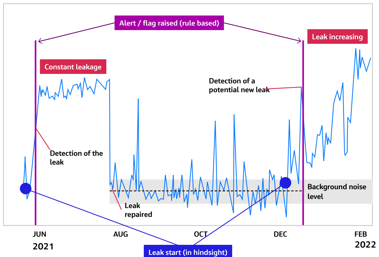
Figure 2 Typical Sotto signal and associated flags
