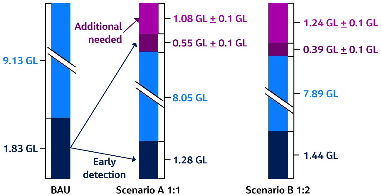
Figure 6 Potential leak savings from the Sotto deployment scenario throughout the SEW network
