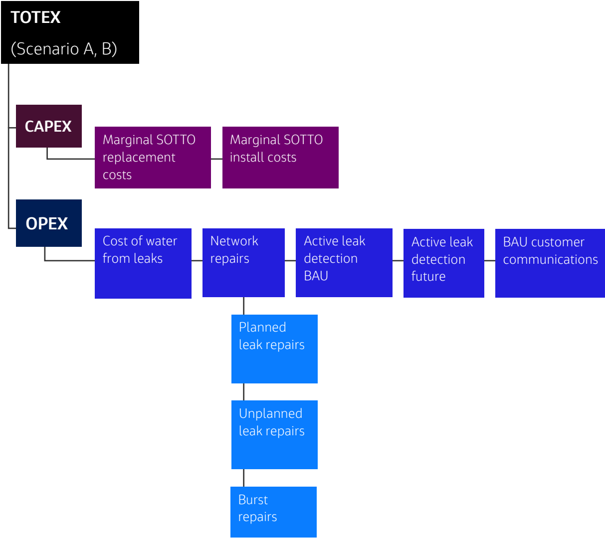
Figure 7 Marginal TOTEX Model economic calculation CAPEX and OPEX components
